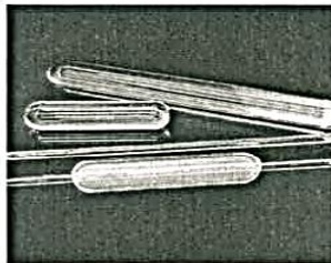
Long form level gauge glasses, reflex and transparent.
