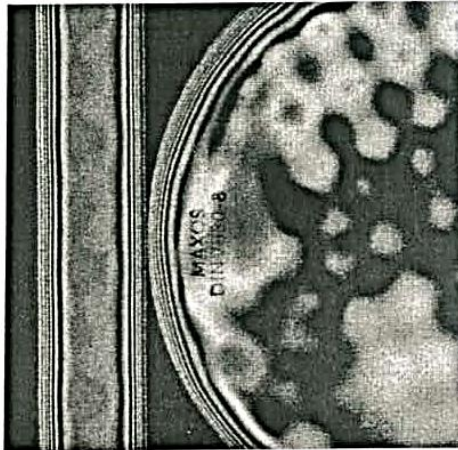
Special tempered MAXOS® glasses under polarised light.
