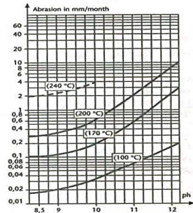
The abrasion of MAXOS®-glass in watery phase for several temperatures as a function of the ph-value.
