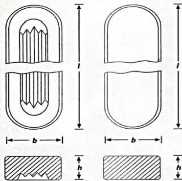
Reflex type glass (R form)
